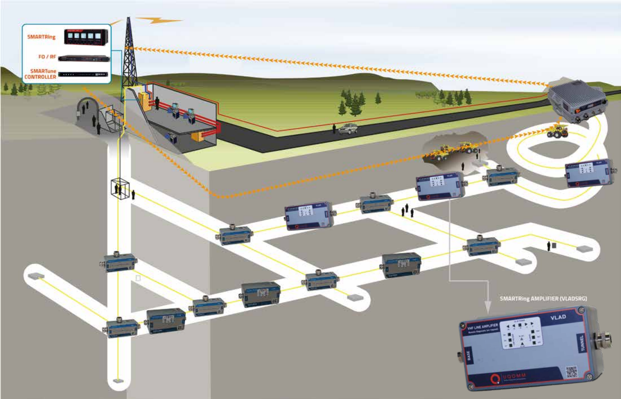
Leaky Feeder SMARTRing: Redundant Leaky Feeder Ring with Fiber Optic
